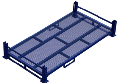
Fine Perforated Base Water permeability: ~54%
